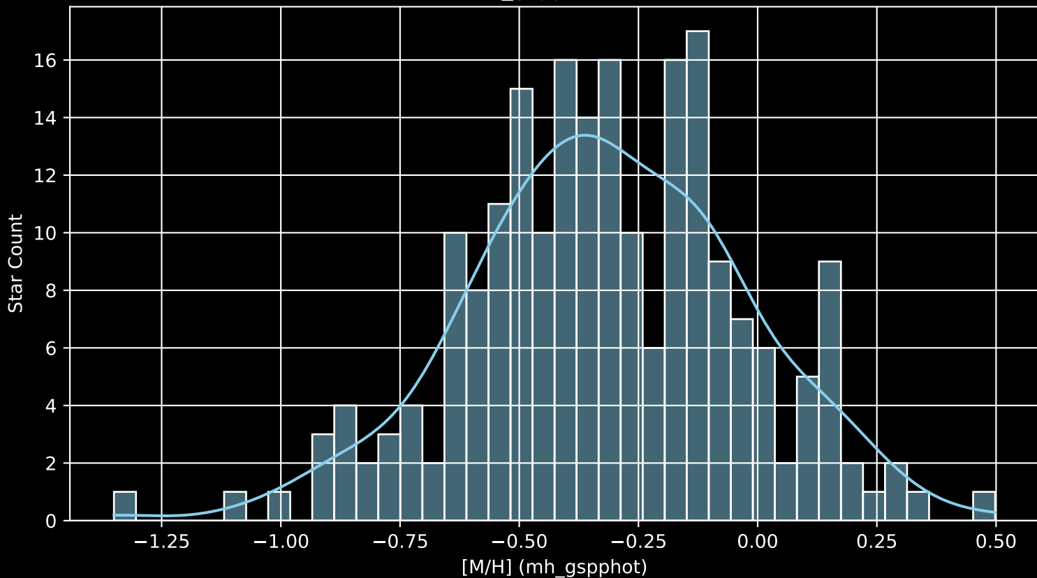
GALAH DR4 Field: [7145] [M/H] (mh_gspphot) (n= 215)
