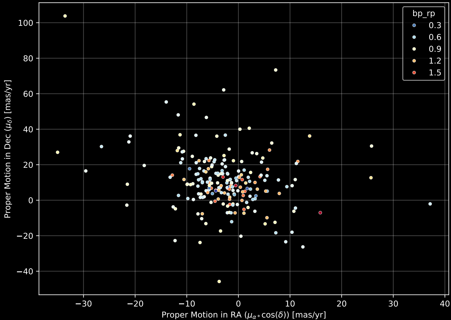
GALAH DR4 Field: [7145] Proper Motion Diagram (n= 215)
