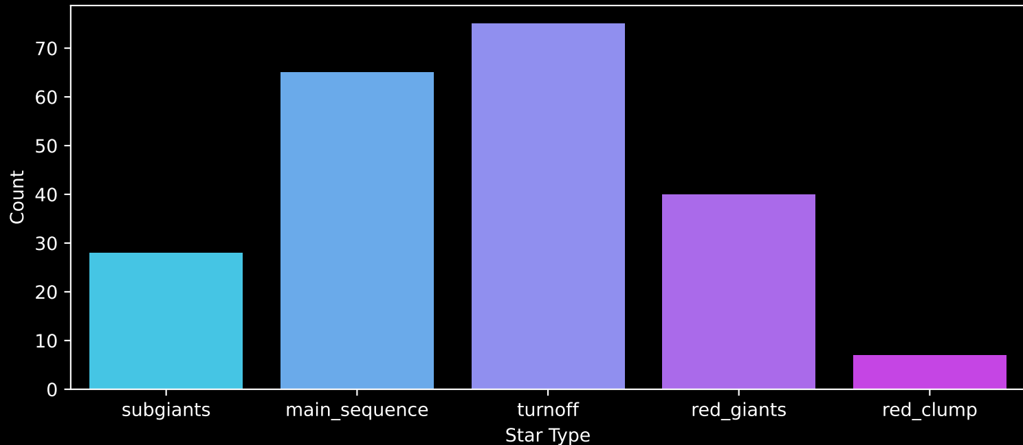
GALAH DR4 Field: [7145] Count plot of Star Type
