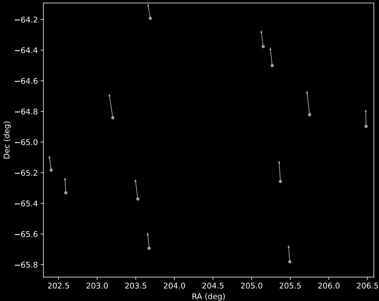
GALAH DR4 Cluster 1 Proper Motion Vectors (n=12)
