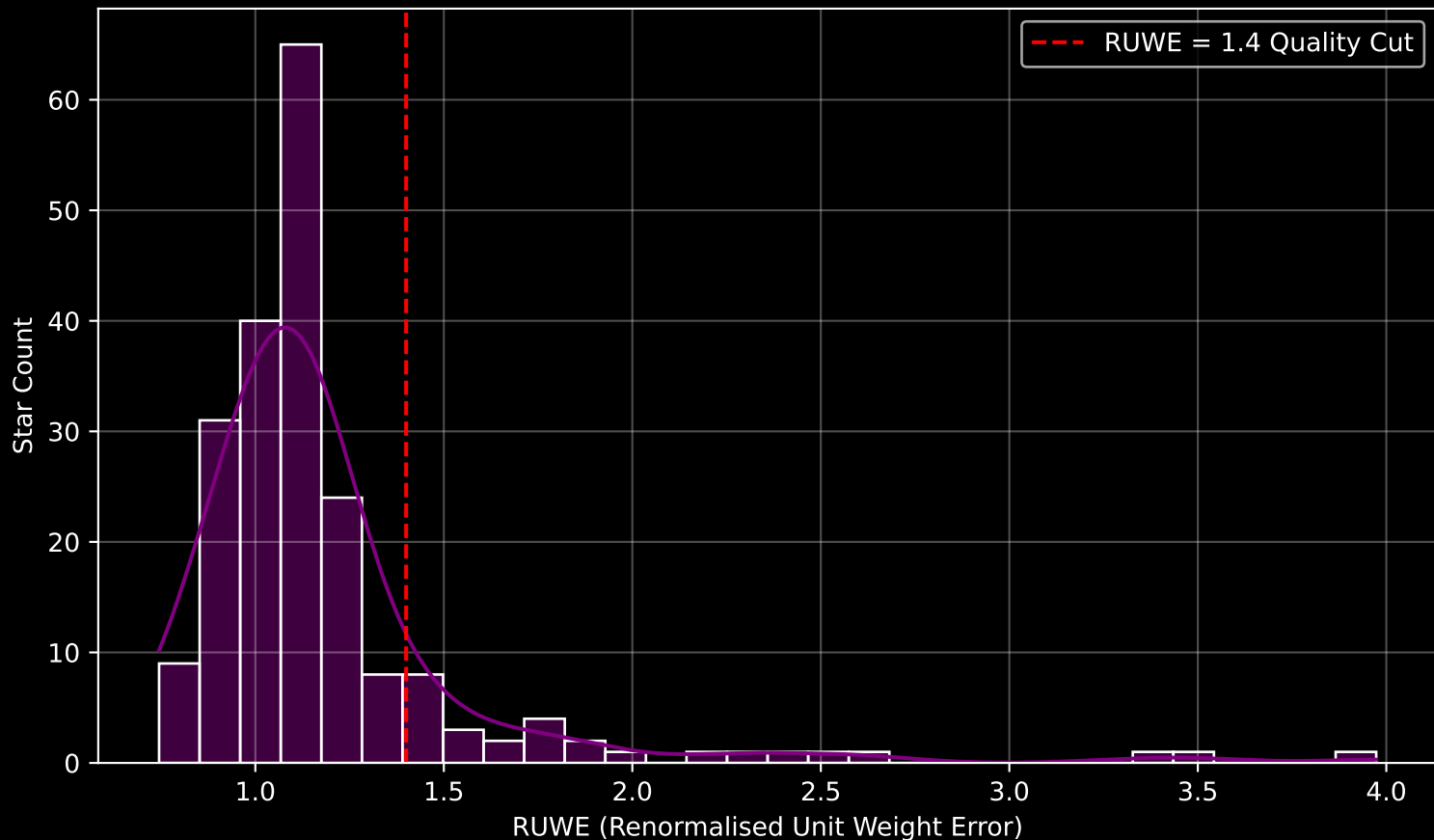
GALAH DR4 Field [7145] RUWE Distribution (n= 205)
