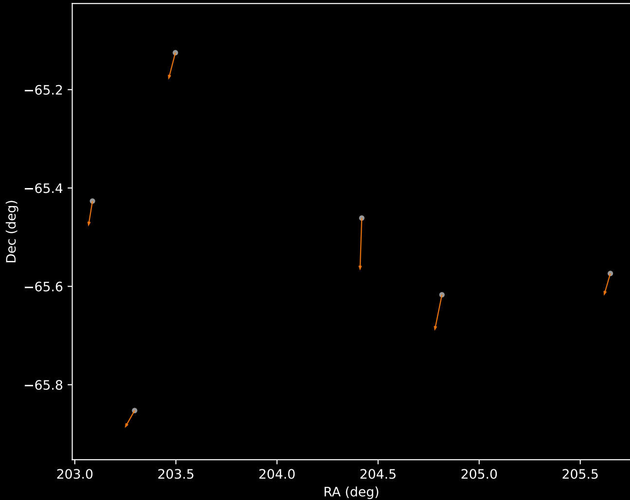
GALAH DR4 Cluster 2 Proper Motion Vectors (n=6)
