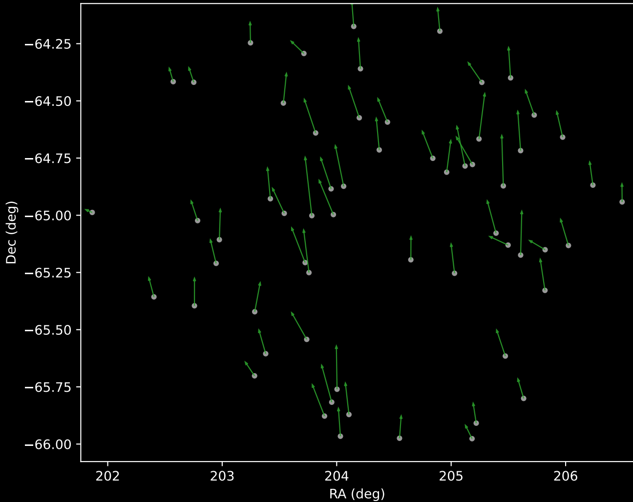
GALAH DR4 Cluster 4 Proper Motion Vectors (n=61)
