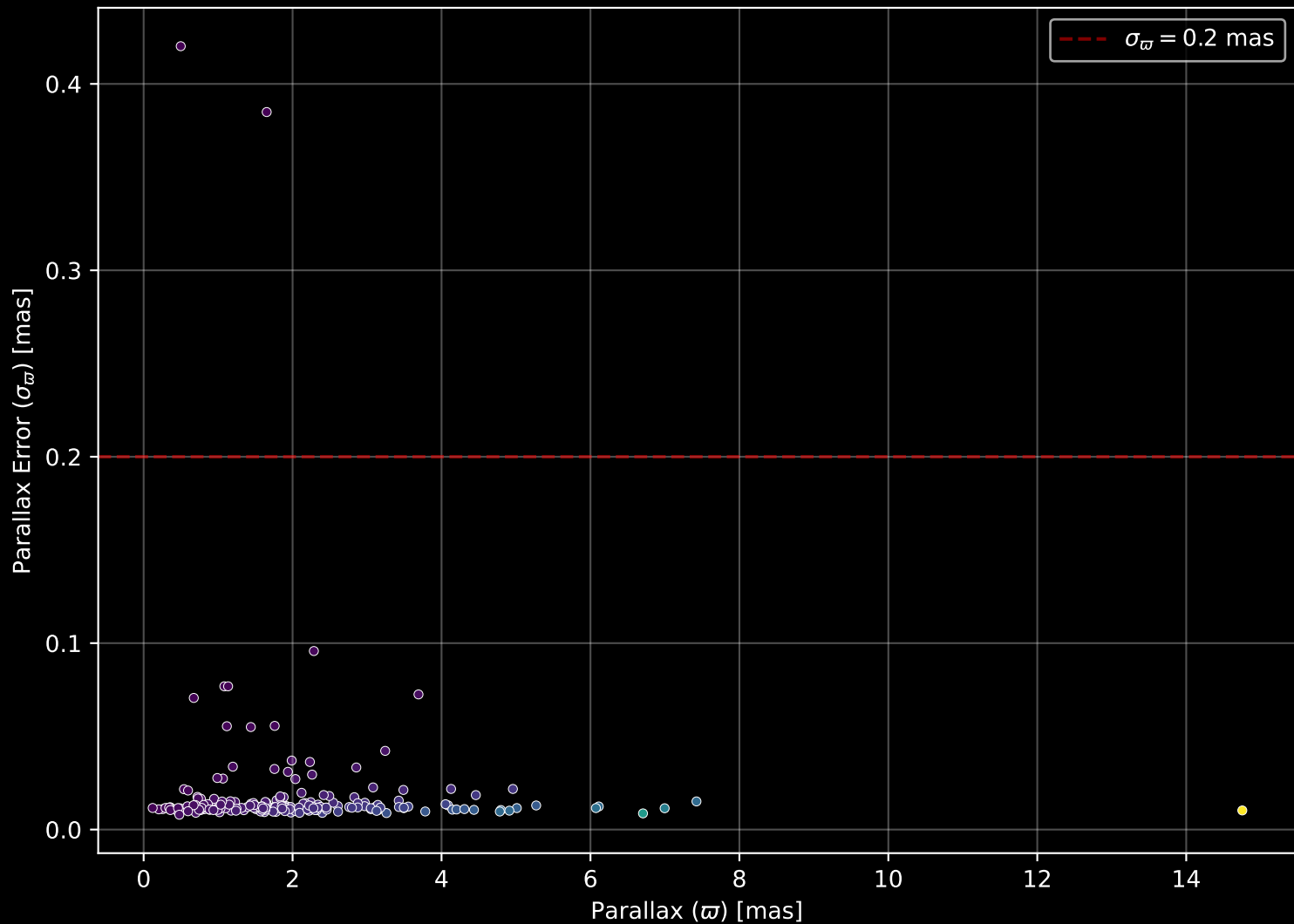
GALAH DR4 Field: [7145] Parallax Quality (n= 215)
