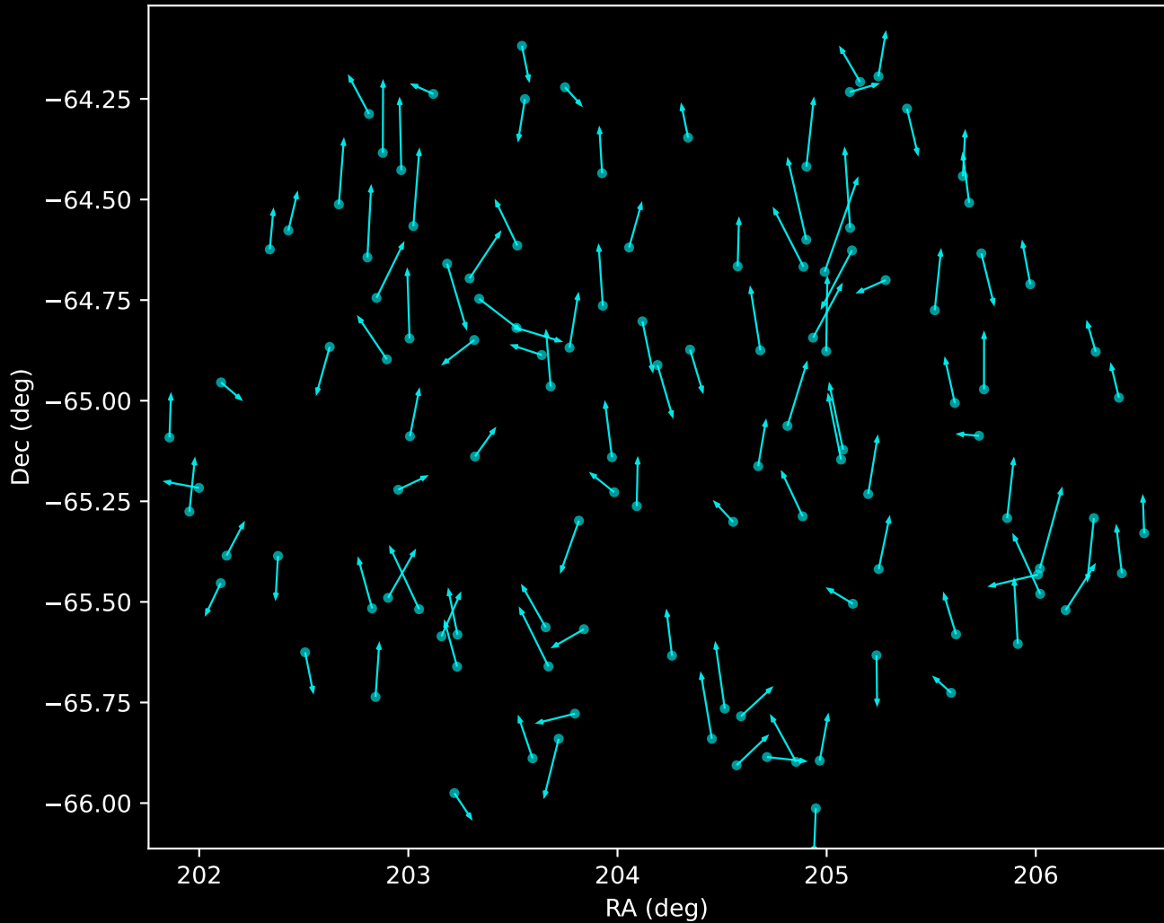
GALAH DR4 Noise Stream Proper Motion Vectors (n=116)
